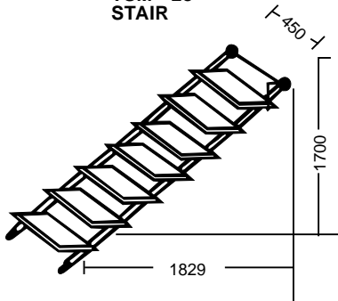
TSM - 28 STAIR
