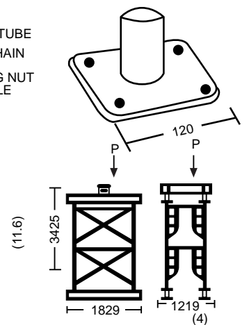
TSM - 30 BASE PLATE
