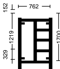
STAIR FRAME 1.70
